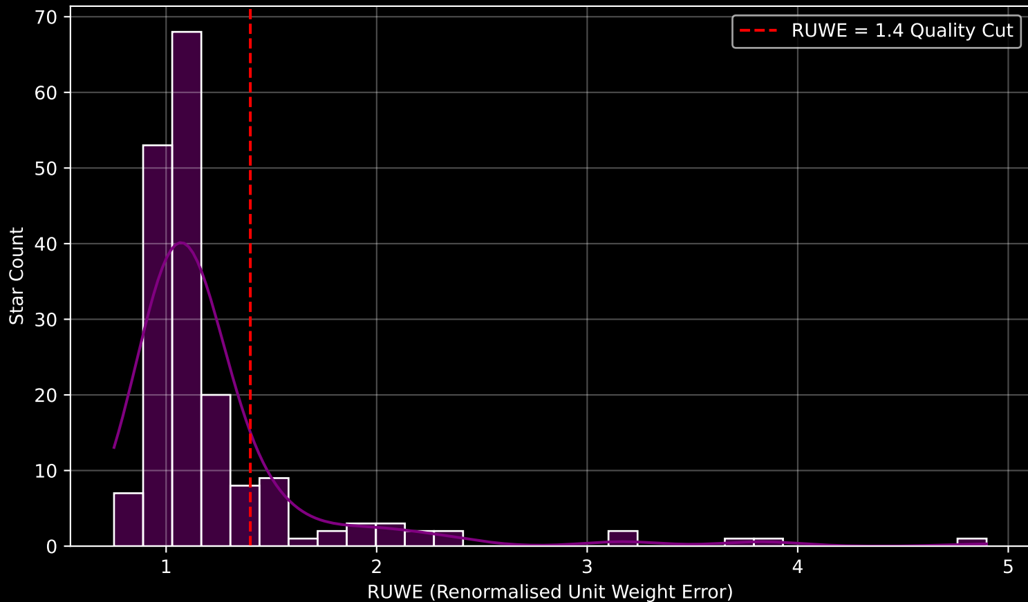
GAPOGEE DR17 Field [Tau_M_MGA] RUWE Distribution (n= 183)
