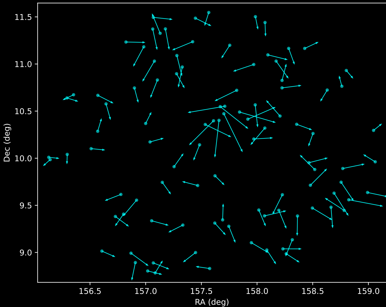
APOGEE DR17 Noise Stream Proper Motion Vectors (n=99)
