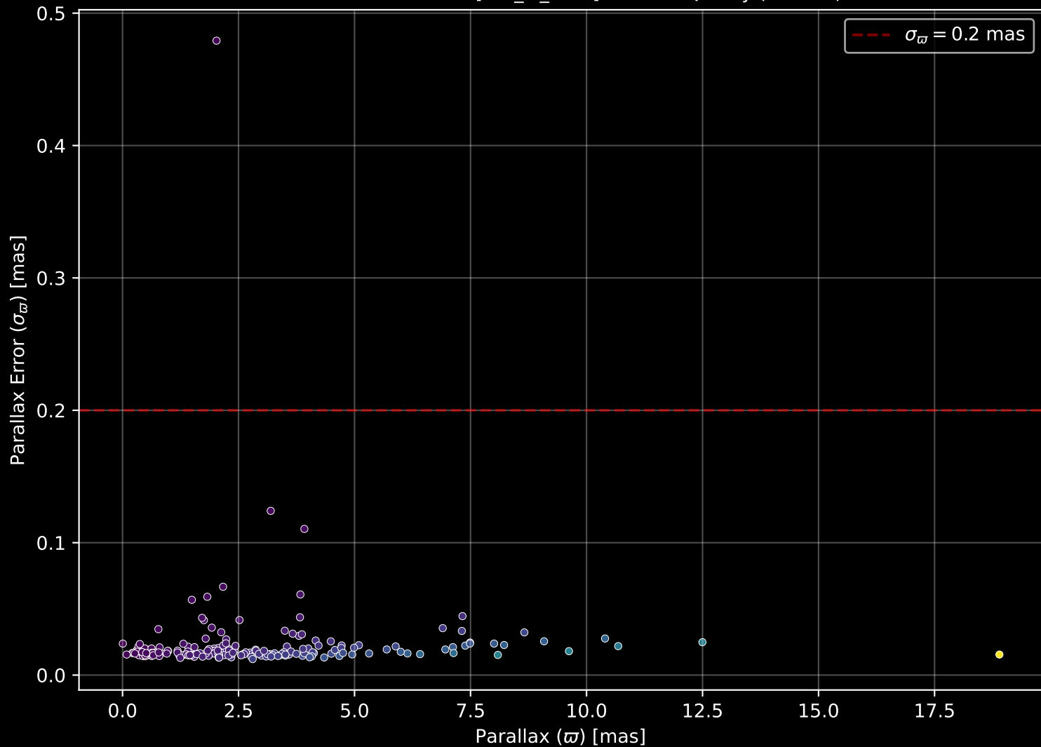
APOGEE DR17 Field: [Tau_M_MGA] Parallax Quality (n= 186)
