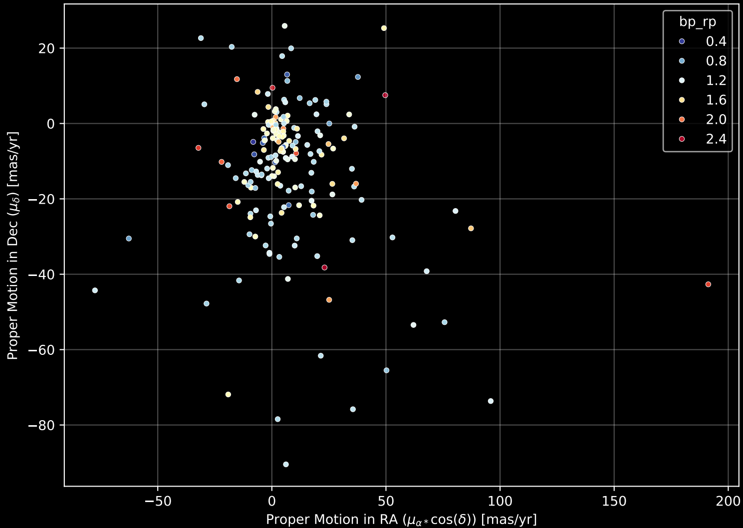
APOGEE DR17 Field: [Tau_M_MGA] Proper Motion Diagram (n= 186)
