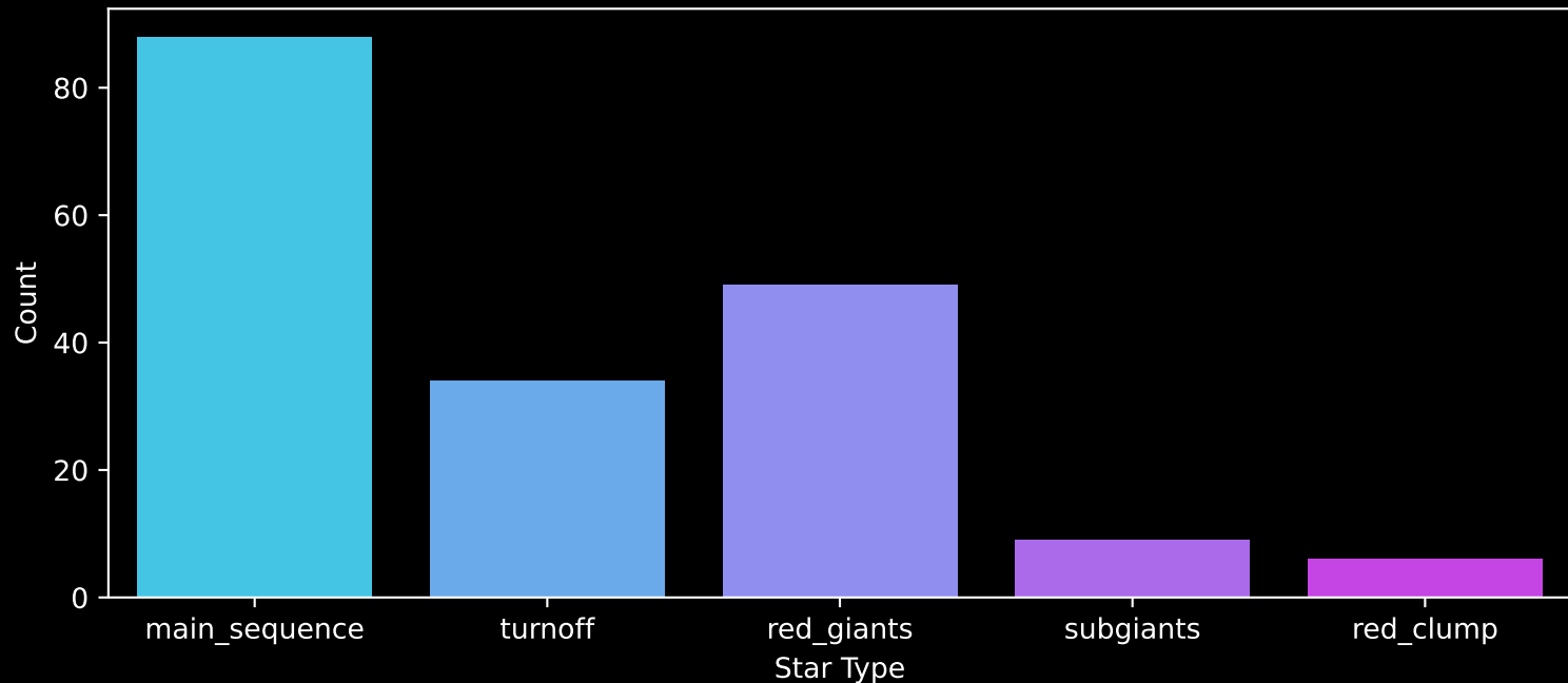
APOGEE DR17 Field: [Tau_M_MGA] Count plot of Star Type
