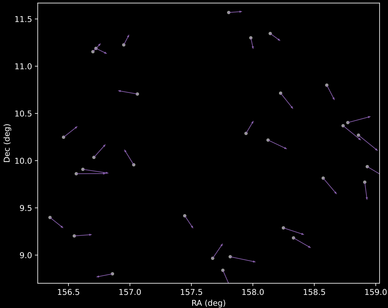
APOGEE DR17 Cluster 8 Proper Motion Vectors (n=31)
