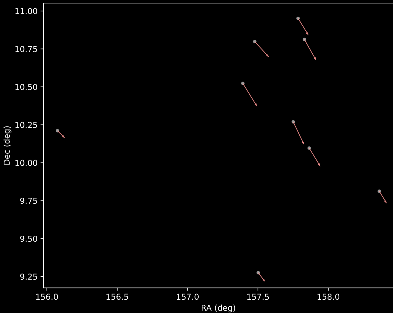
APOGEE DR17 Cluster 7 Proper Motion Vectors (n=9)
