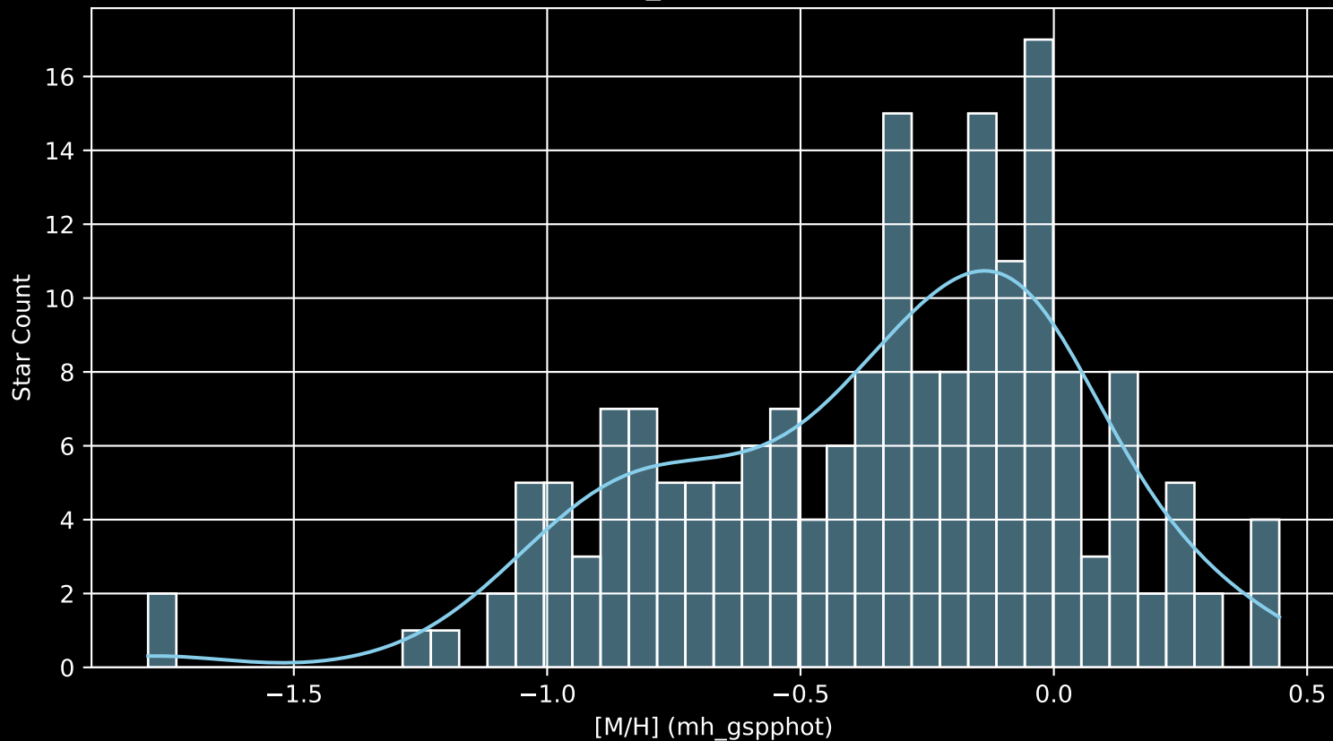
APOGEE DR17 Field: [Tau_M_MGA [M/H] (mh_gspphot) (n= 185)
